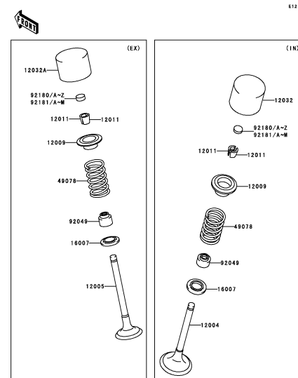
B-8 Valve(s)(1/2)
