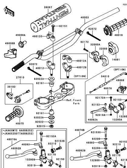
F-7 Handlebar(1/2)
