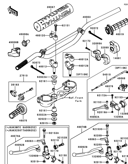
F-8 Handlebar(2/2)
