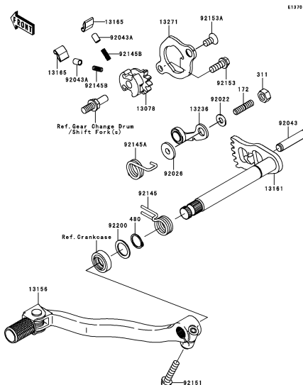
C-4 Gear Change Mechanism
