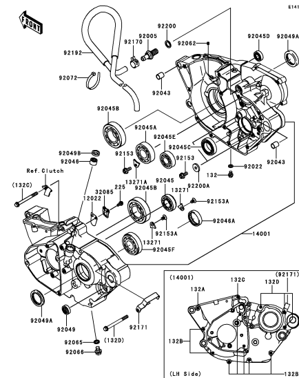
C-5 Crankcase
