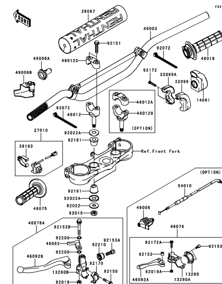
F-8 Handlebar(2/2)
