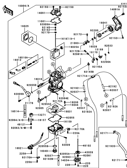
C-7 Carburetor(1/4)
