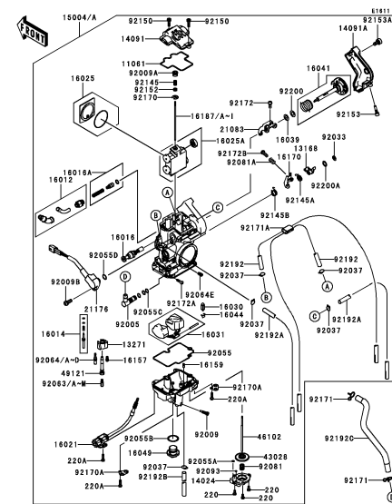
C-8 Carburetor(2/4)
