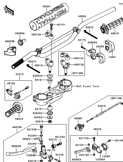
F-7 Handlebar(1/2)
