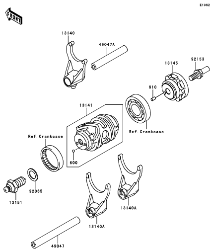
C-3 Gear Change Drum/Shift Fork(s)
