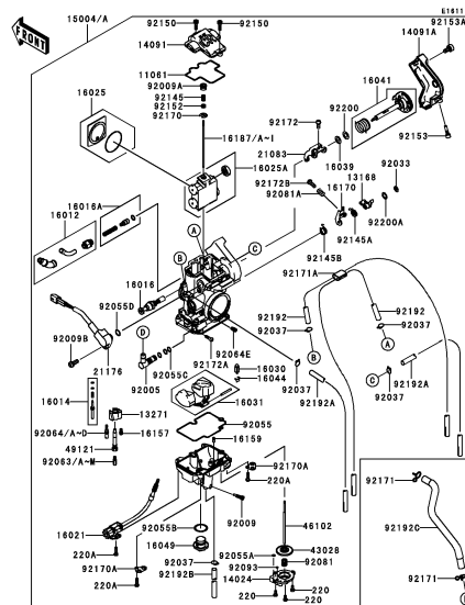
C-10 Carburetor(4/4)
