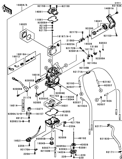
C-9 Carburetor(3/4)
