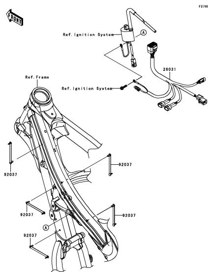
G-3 Chassis Electrical Equipment
