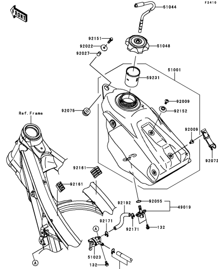
F-11 Fuel Tank
