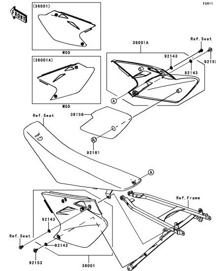
F-14 Side Covers
