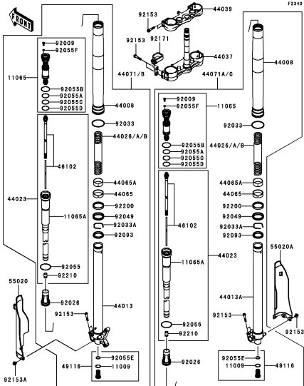
F-9 Front Fork(1/2)
