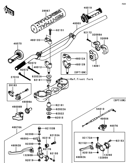
F-7 Handlebar(1/2)
