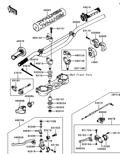
F-8 Handlebar(2/2)
