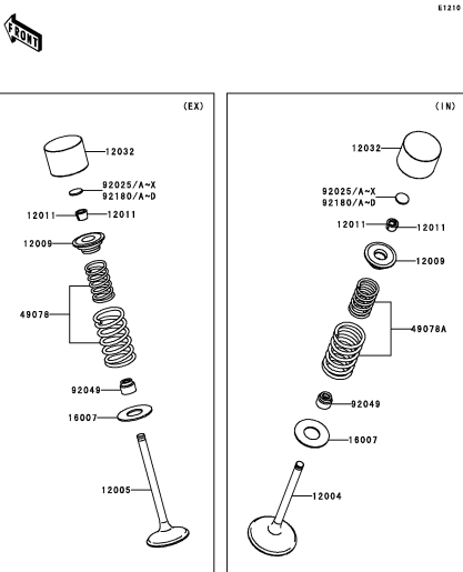
B-8 Valve(s)
