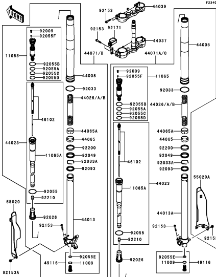
F-10 Front Fork(2/2)
