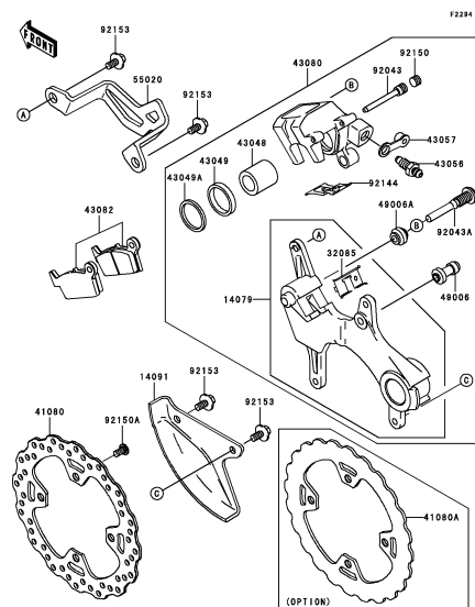
F-6 Rear Brake
