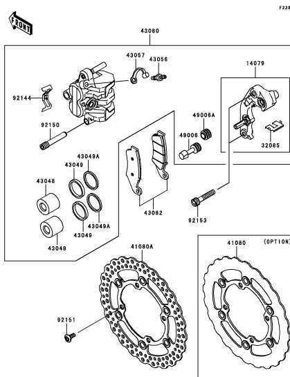
F-4 Front Brake
