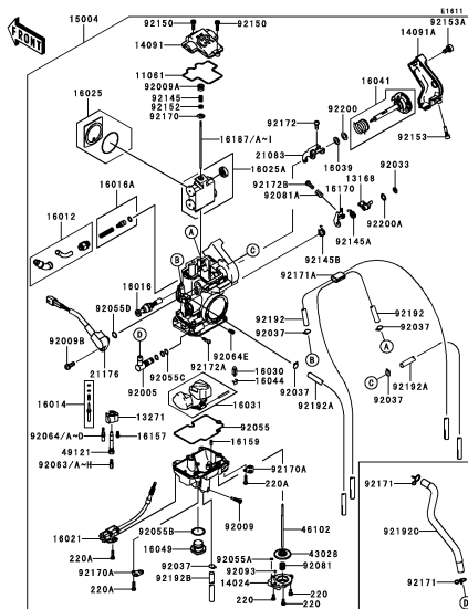
C-9 Carburetor(2/3)
