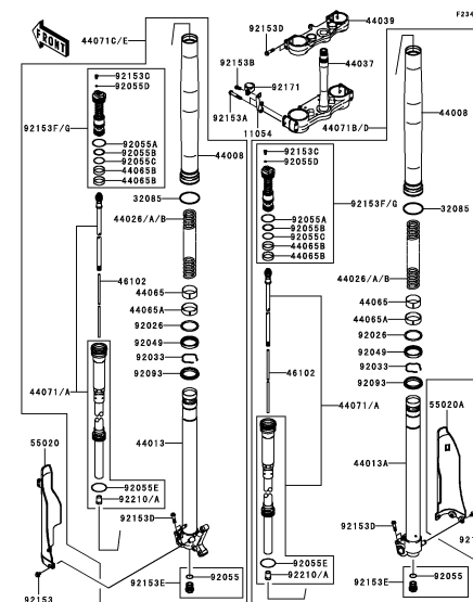
F-11 Front Fork(2/2)
