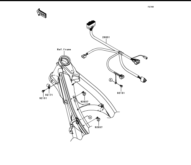
G-4 Chassis Electrical Equipment
