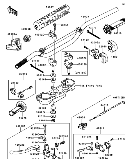
F-8 Handlebar(1/2)
