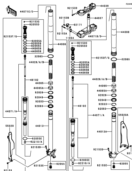
F-10 Front Fork(1/2)
