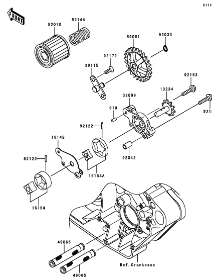
C-11 Oil Pump
