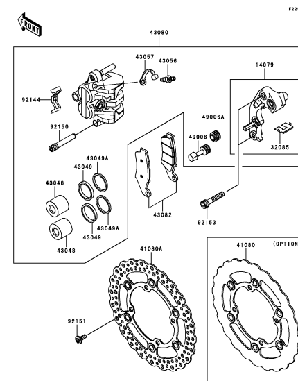
F-5 Front Brake
