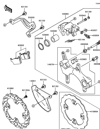
F-7 Rear Brake
