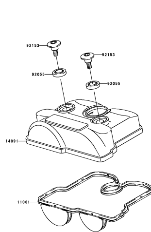
B-4 Cylinder Head Cover
