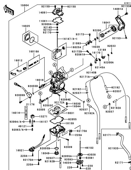
C-10 Carburetor(3/3)
