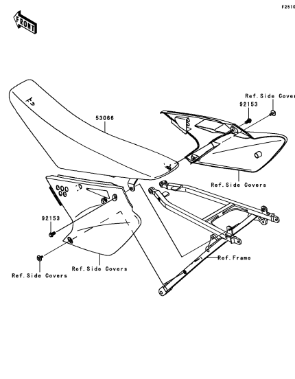
F-13 Seat
