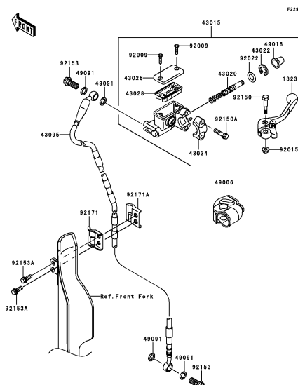
F-4 Front Master Cylinder
