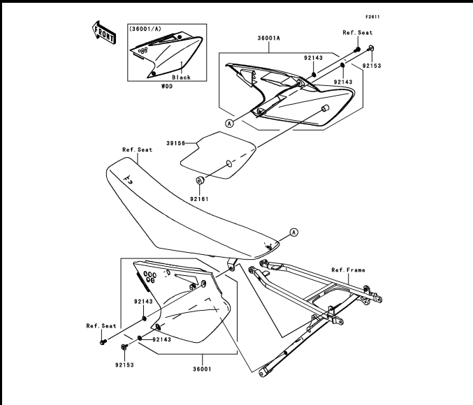
G-3 Side Covers
