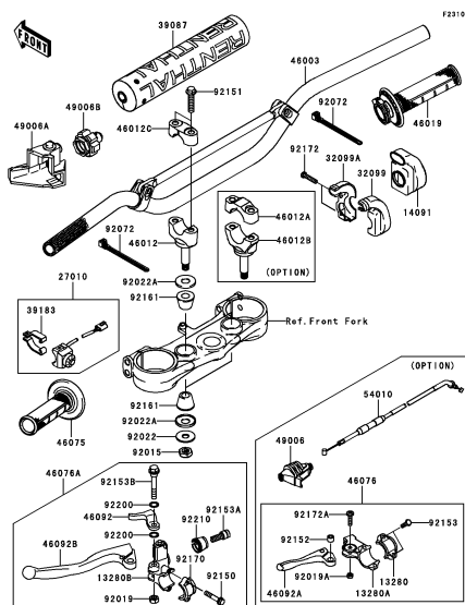
F-9 Handlebar(2/2)
