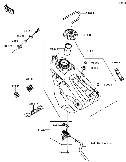
F-12 Fuel Tank
