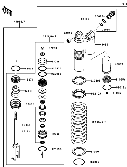
F-3 Shock Absorber(s)
