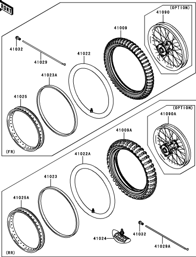
D-10 Tires
