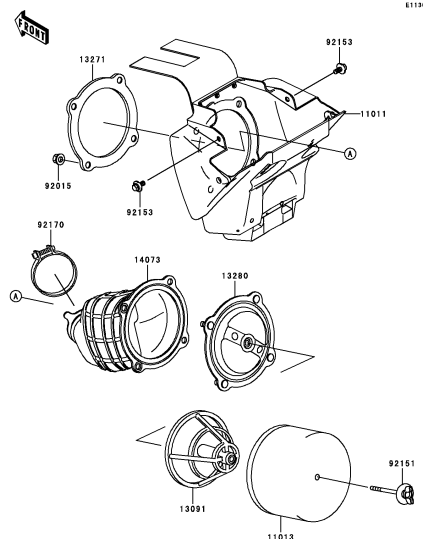
B-4 Air Cleaner
