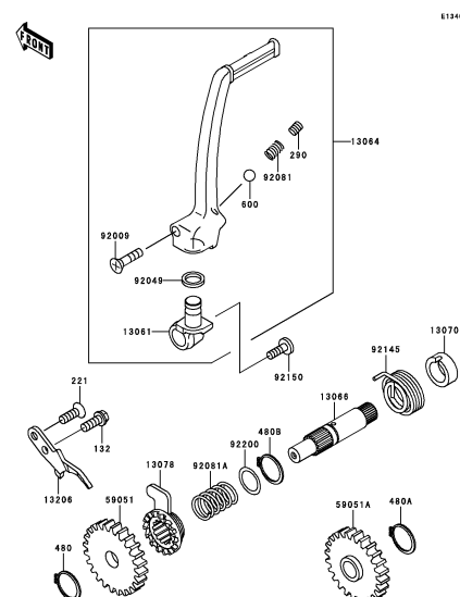
B-7 Kickstarter Mechanism
