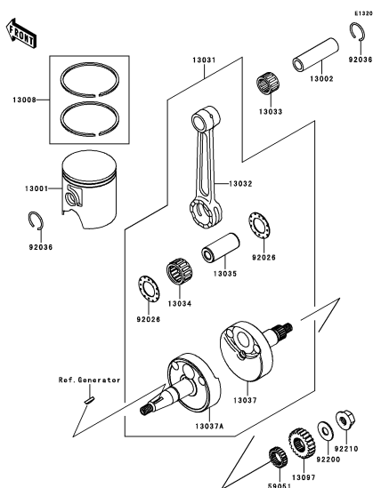
B-6 Crankshaft/Piston(s)
