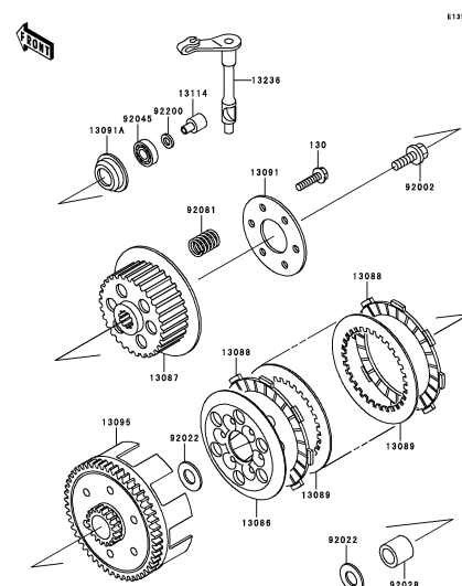
B-8 Clutch
