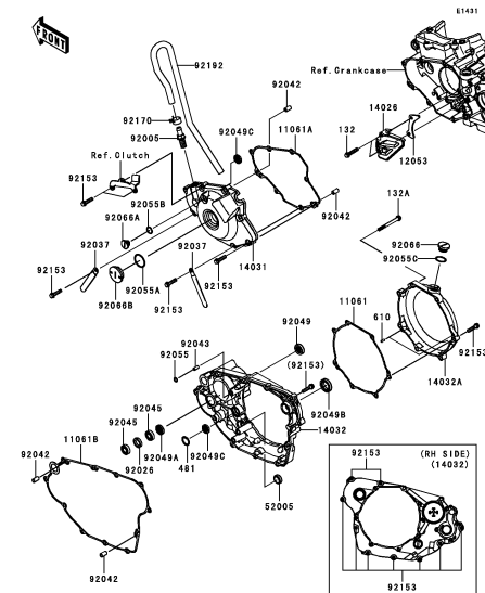
C-5 Engine Cover(s)
