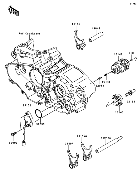
B-14 Gear Change Drum/Shift Fork(s)
