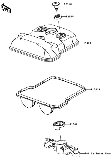
B-4 Cylinder Head Cover
