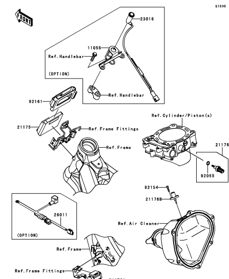
C-8 Fuel Injection
