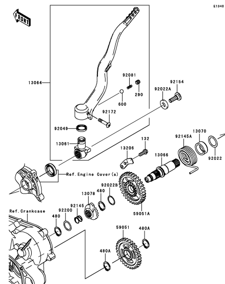
B-11 Kickstarter Mechanism
