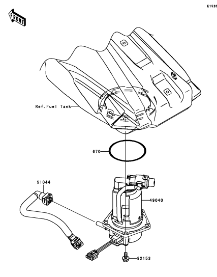
C-7 Fuel Pump
