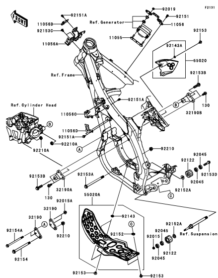
E-4 Frame Fittings
