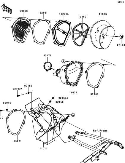
B-6 Air Cleaner
