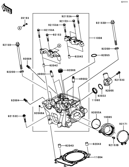
B-3 Cylinder Head
