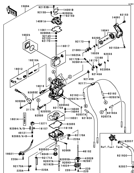
C-10 Carburetor(3/3)
