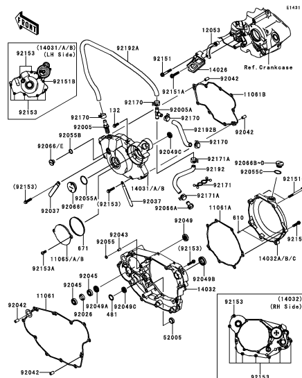
C-6 Engine Cover(s)(1/2)
