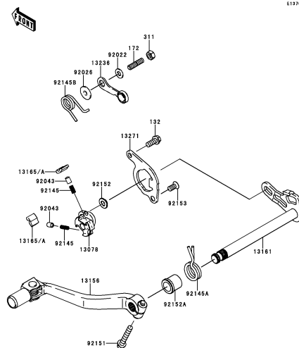
C-4 Gear Change Mechanism
