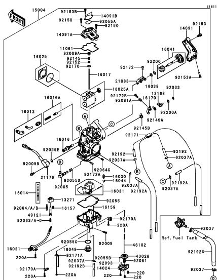
C-9 Carburetor(2/3)
