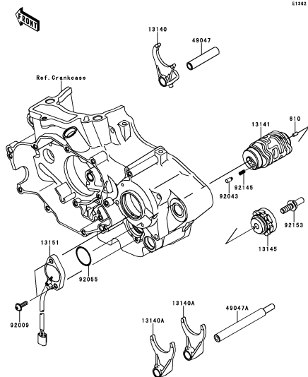
C-3 Gear Change Drum/Shift Fork(s)
