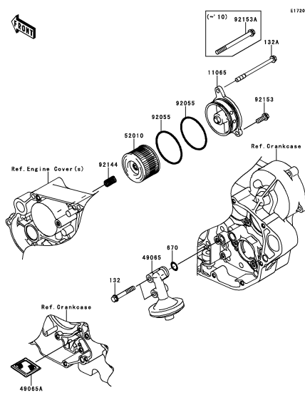
C-12 Oil Filter
