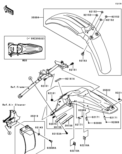
E-9 Fenders
