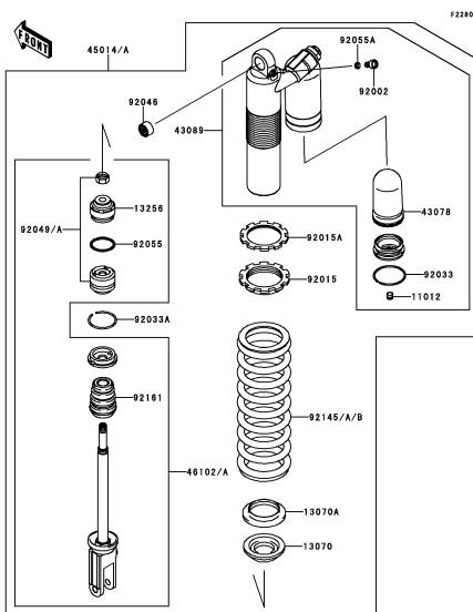
F-3 Shock Absorber(s)
