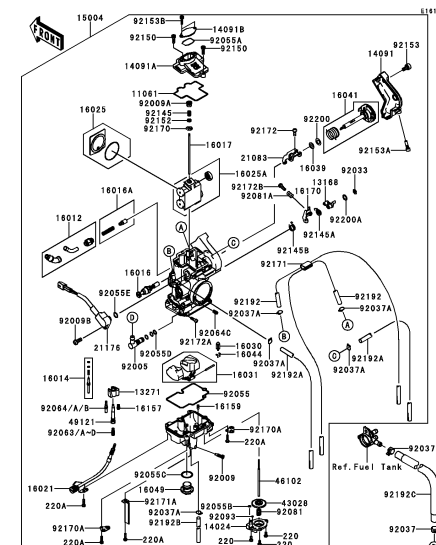
C-8 Carburetor(1/3)
