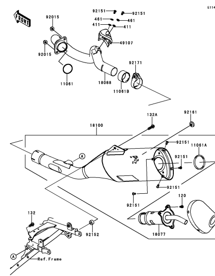
B-8 Muffler(s)(JKALX450AAA006446~)
