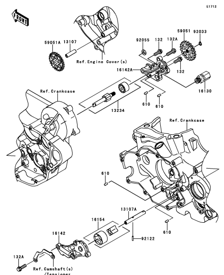
C-11 Oil Pump
