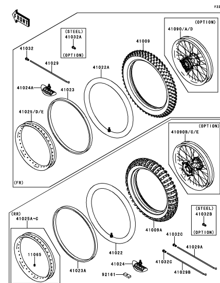
E-11 Tires
