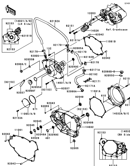
C-7 Engine Cover(s)(2/2)
