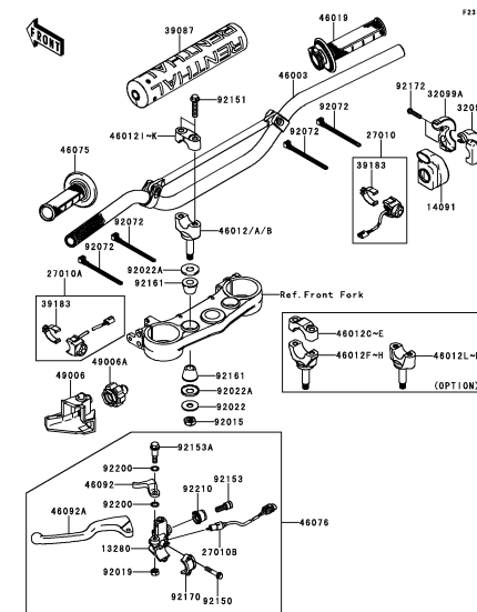
F-8 Handlebar(1/2)
