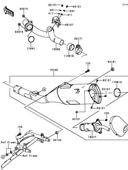
B-7 Muffler(s)(~JKALX450AAA006445)
