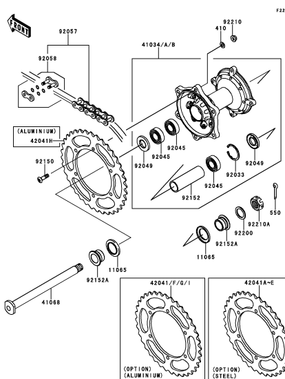
E-13 Rear Hub
