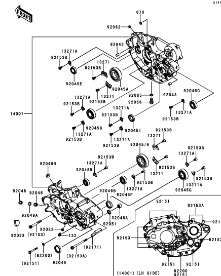
C-5 Crankcase
