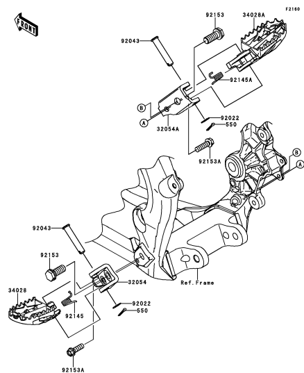
D-8 Footrests
