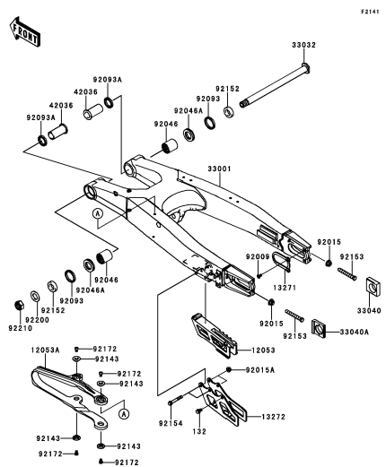
D-6 Swingarm
