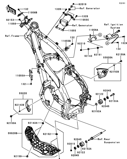
D-5 Frame Fittings
