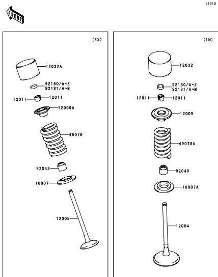
B-8 Valve(s)(1/2)
