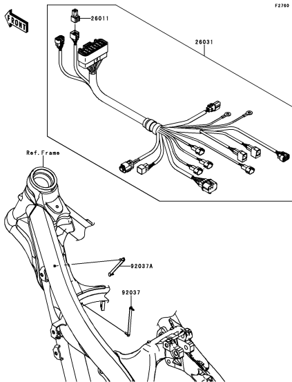
F-3 Chassis Electrical Equipment
