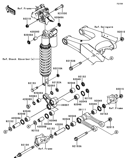
D-7 Suspension
