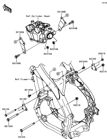
D-4 Engine Mount
