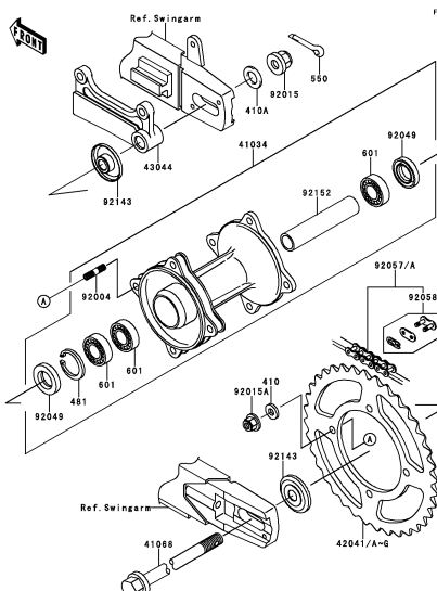
D-13 Rear Hub
