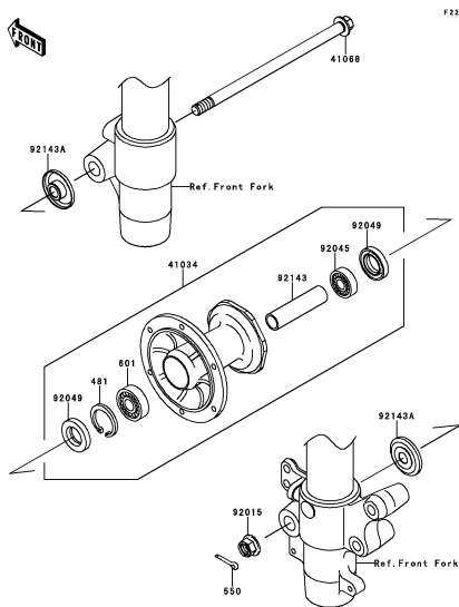
D-12 Front Hub
