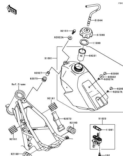
E-11 Fuel Tank
