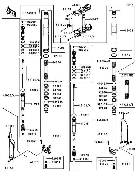
F-9 Front Fork(2/2)
