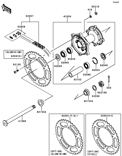
E-12 Rear Hub
