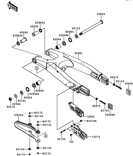
E-5 Swingarm
