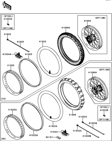
E-10 Tires
