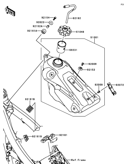
F-10 Fuel Tank
