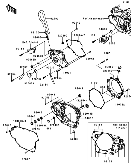
Engine Cover(s)
