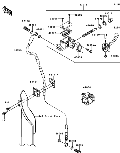
F-3 Front Master Cylinder
