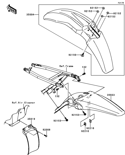
E-8 Fenders
