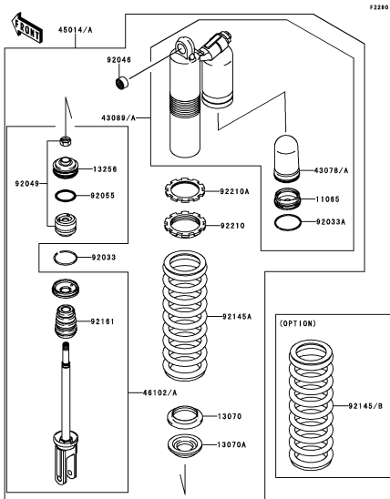
E-14 Shock Absorber(s)
