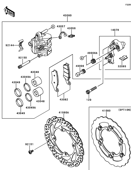
F-4 Front Brake
