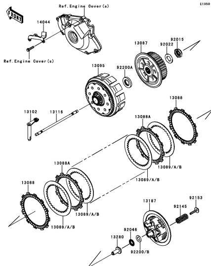
B-12 Clutch
