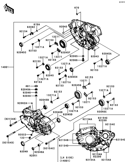
Crankcase
