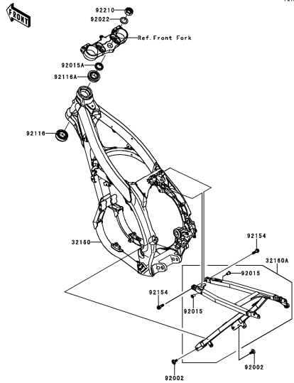
E-3 Frame
