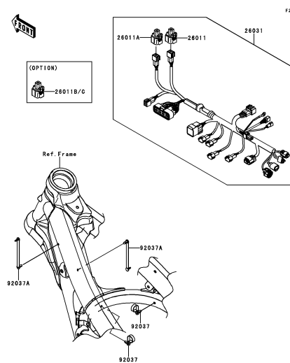
F-14 Chassis Electrical Equipment
