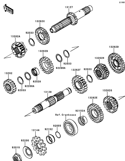
B-13 Transmission
