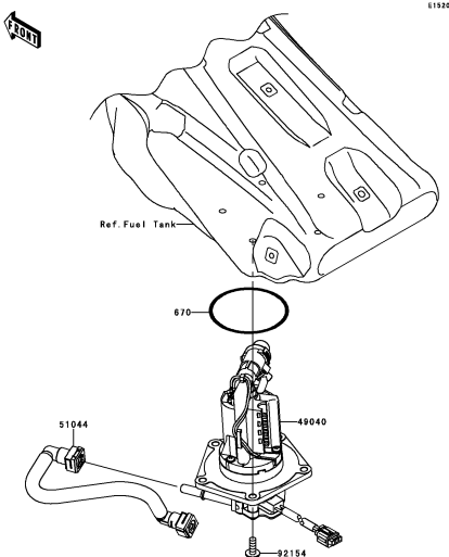
Fuel Pump
