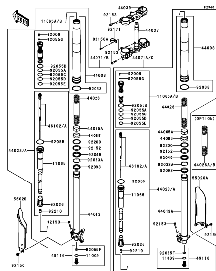
F-8 Front Fork(1/2)
