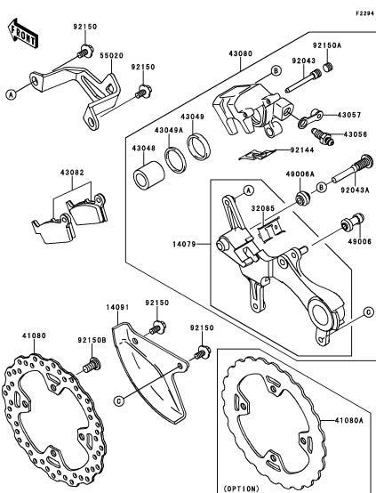
F-6 Rear Brake
