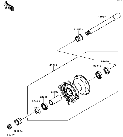
E-11 Front Hub
