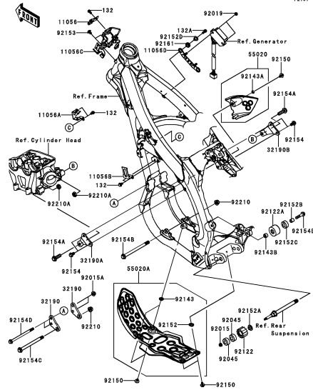
E-4 Frame Fittings
