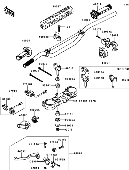
F-7 Handlebar
