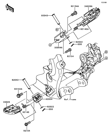
E-7 Footrests
