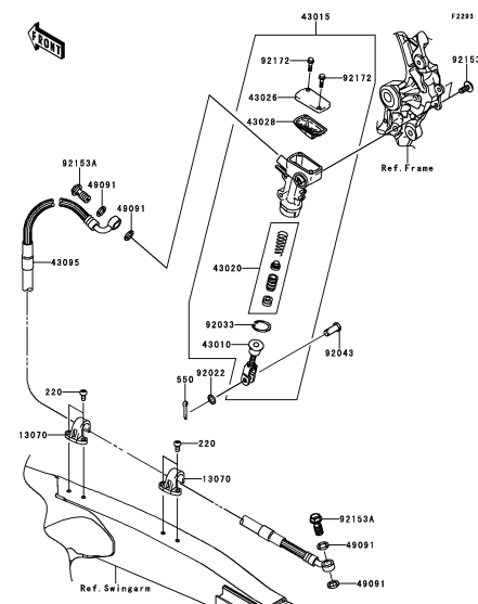
F-5 Rear Master Cylinder
