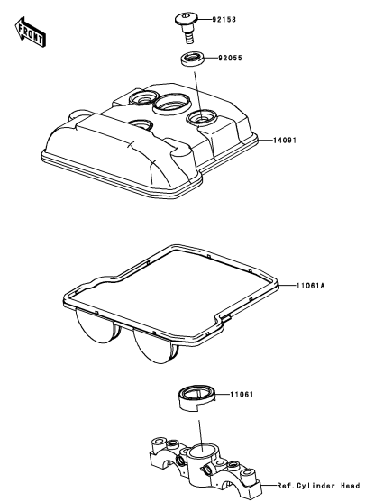
B-4 Cylinder Head Cover
