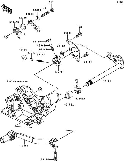
Gear Change Mechanism
