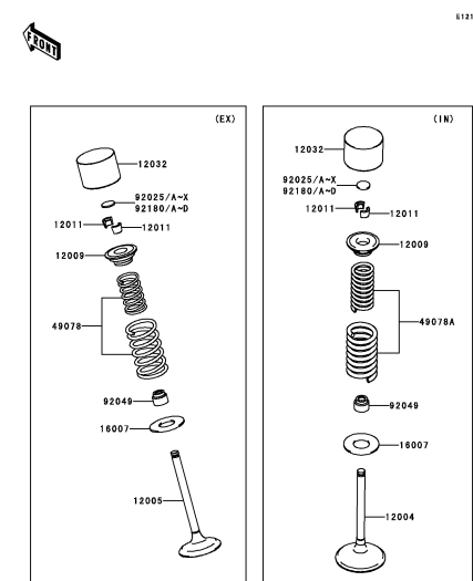
B-8 Valve(s)
