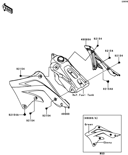
D-3 Engine Shrouds
