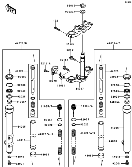
E-9 Front Fork(2/2)
