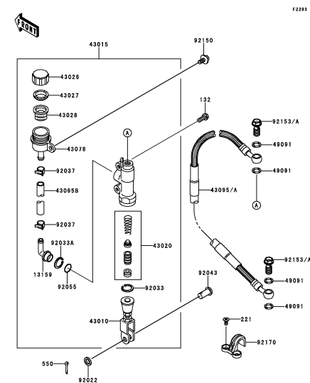
E-5 Rear Master Cylinder
