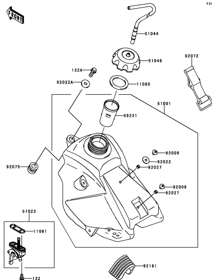
E-10 Fuel Tank
