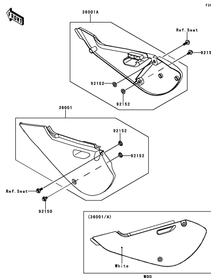
E-13 Side Covers
