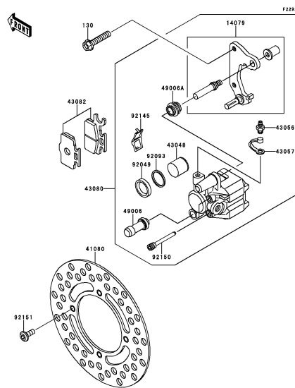
E-4 Front Brake
