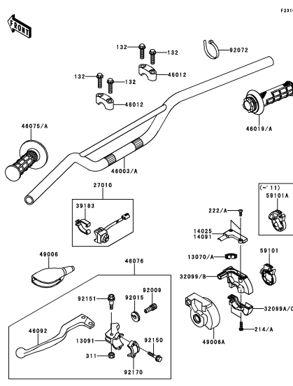
E-7 Handlebar
