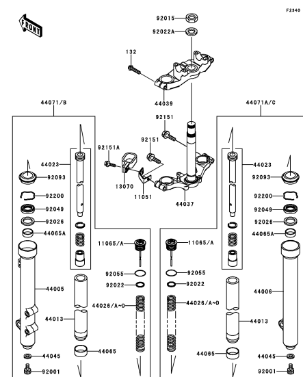
E-8 Front Fork(1/2)
