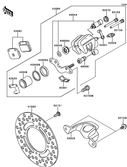
E-6 Rear Brake
