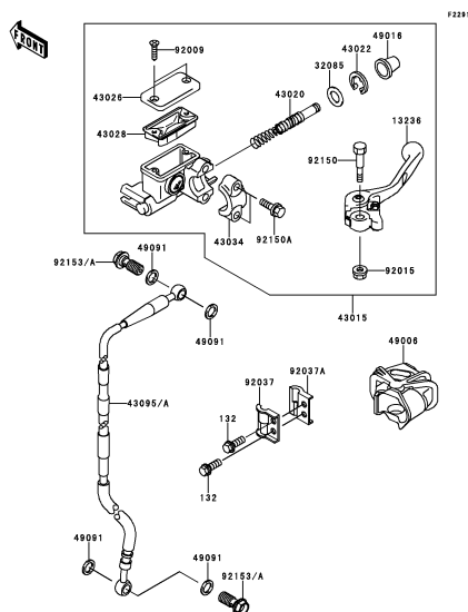
E-3 Front Master Cylinder
