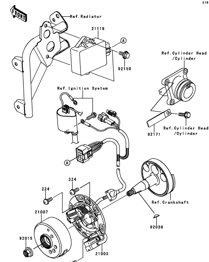
C-5 Generator
