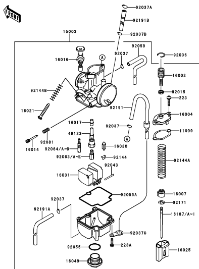
C-3 Carburetor(1/2)
