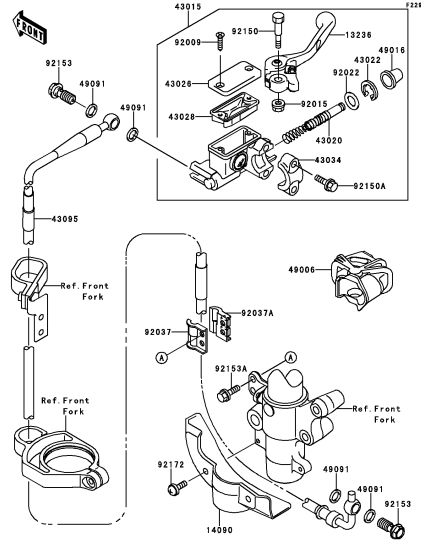
E-4 Front Master Cylinder
