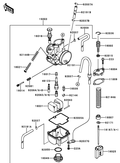
C-4 Carburetor(2/2)
