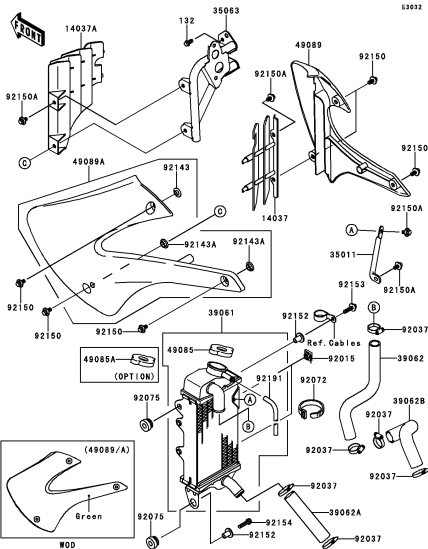
C-7 Radiator
