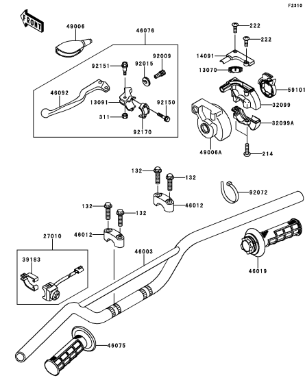
E-8 Handlebar
