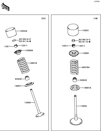
B-9 Valve(s)(2/2)
