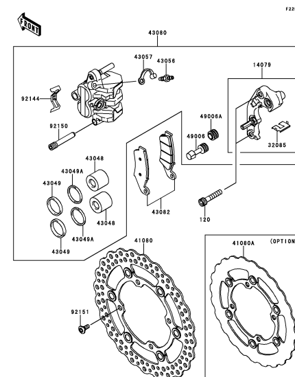
E-5 Front Brake
