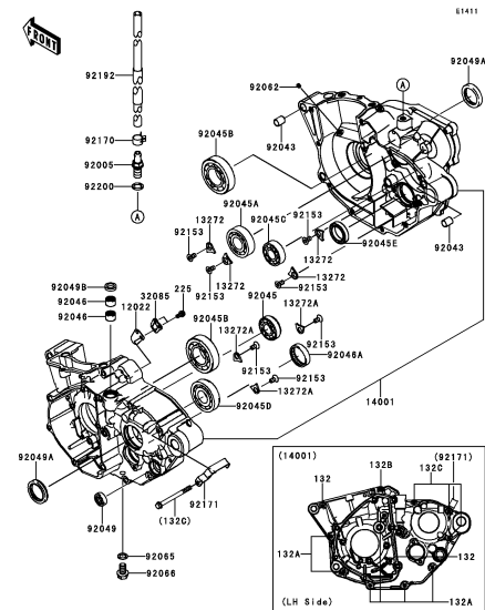
C-5 Crankcase
