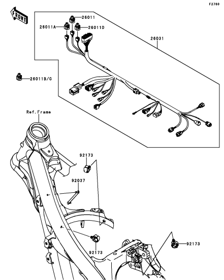
E-14 Chassis Electrical Equipment
