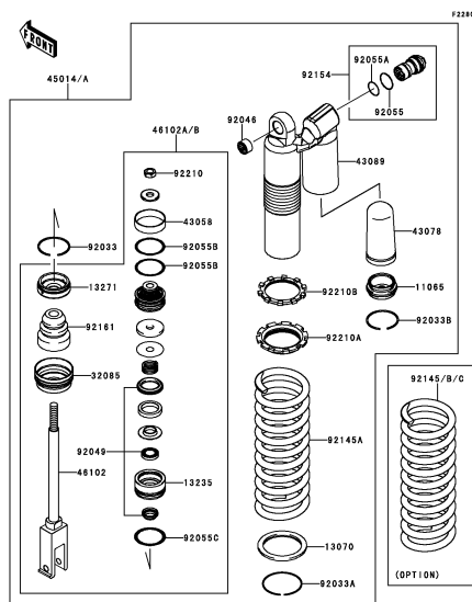
E-3 Shock Absorber(s)
