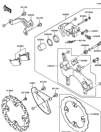
E-7 Rear Brake
