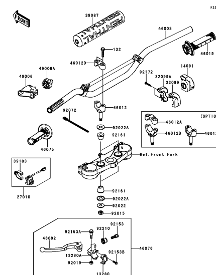
E-8 Handlebar
