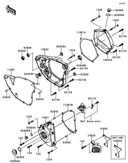
C-6 Engine Cover(s)
