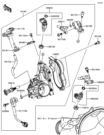
C-7 Throttle
