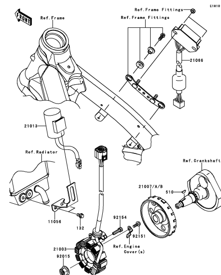
C-11 Generator
