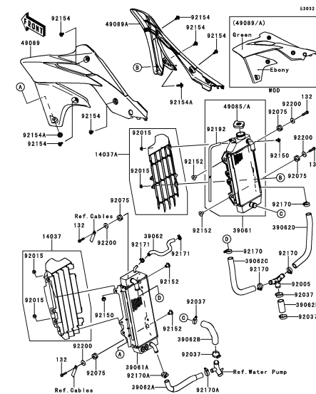
C-14 Radiator
