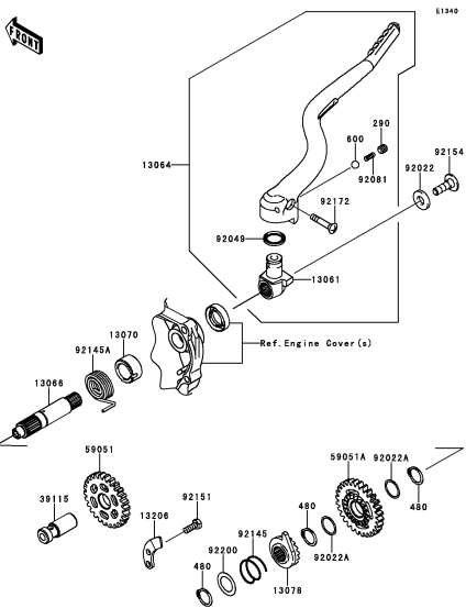
B-12 Kickstarter Mechanism
