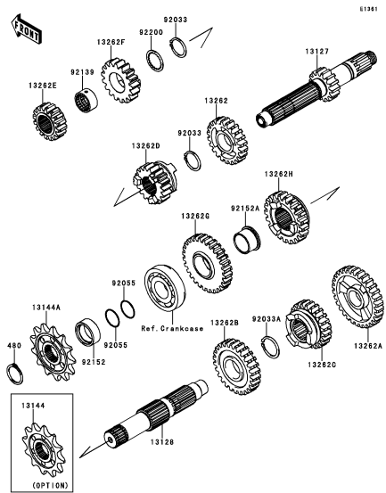
B-14 Transmission
