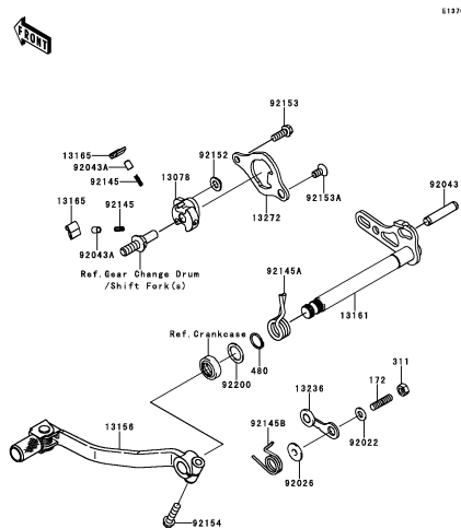
C-4 Gear Change Mechanism
