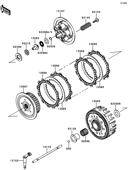
B-13 Clutch
