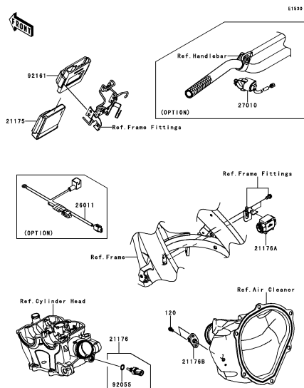
C-9 Fuel Injection
