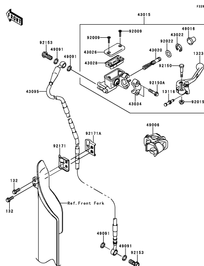
E-4 Front Master Cylinder
