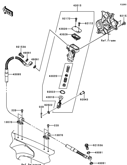
E-6 Rear Master Cylinder
