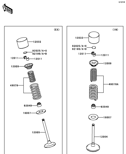
B-8 Valve(s)
