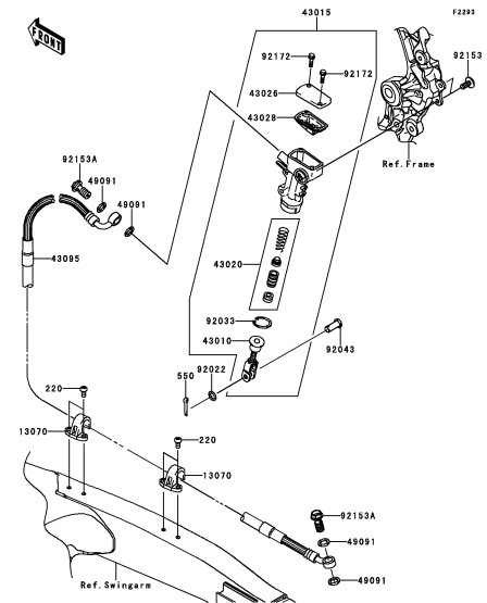
F-5 Rear Master Cylinder
