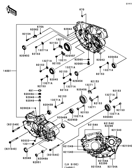
C-4 Crankcase
