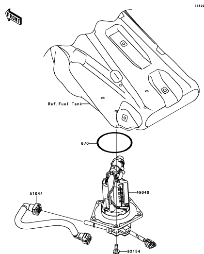
C-7 Fuel Pump
