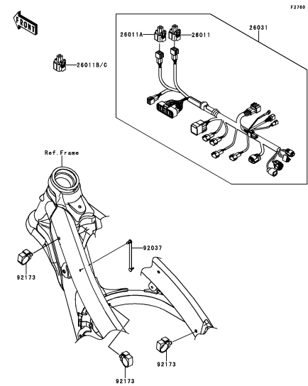
F-14 Chassis Electrical Equipment
