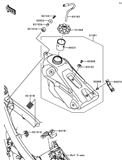
F-10 Fuel Tank
