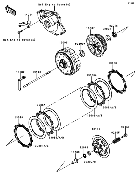
B-12 Clutch
