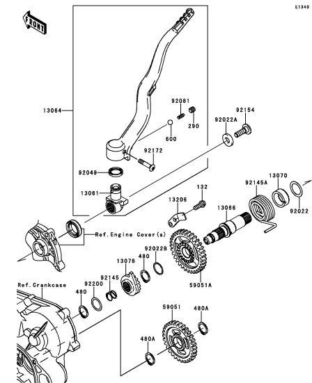
B-11 Kickstarter Mechanism
