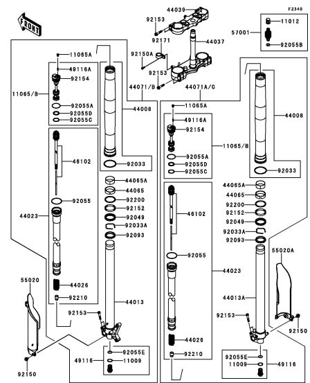
F-8 Front Fork(1/2)
