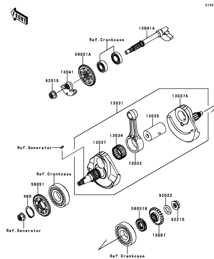
B-10 Crankshaft
