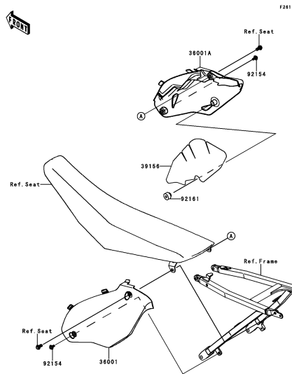
F-13 Side Covers
