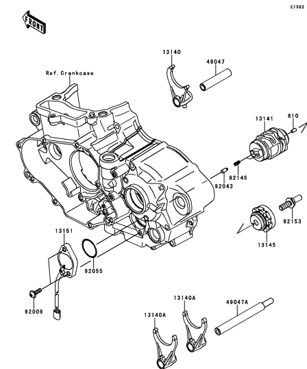
B-14 Gear Change Drum/Shift Fork(s)
