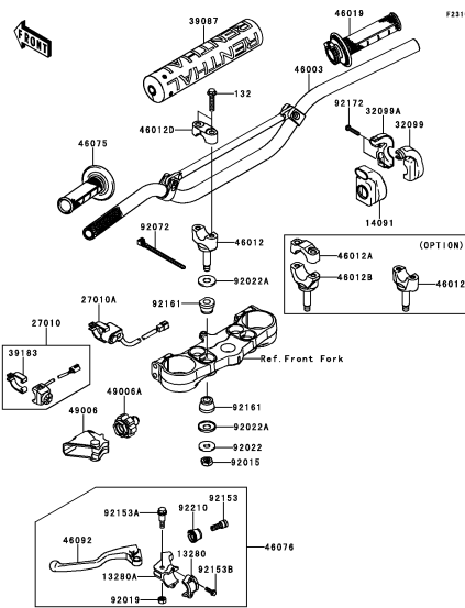
F-7 Handlebar
