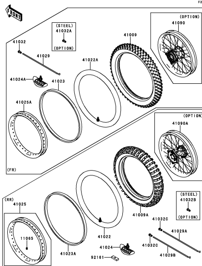
E-10 Tires
