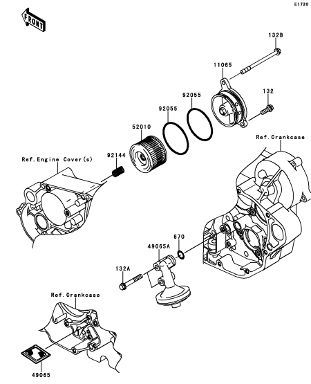
C-11 Oil Filter
