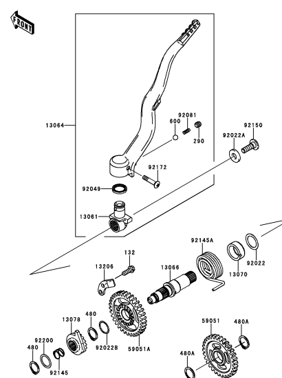
B-11 Kickstarter Mechanism
