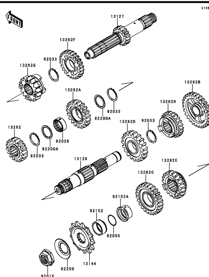
B-13 Transmission
