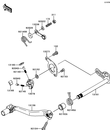
C-3 Gear Change Mechanism
