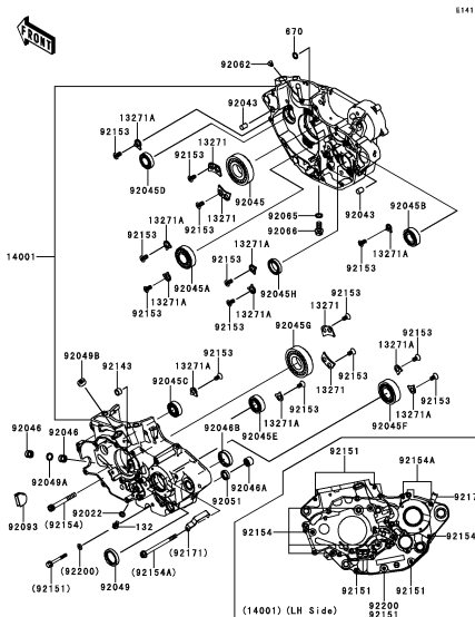
C-4 Crankcase
