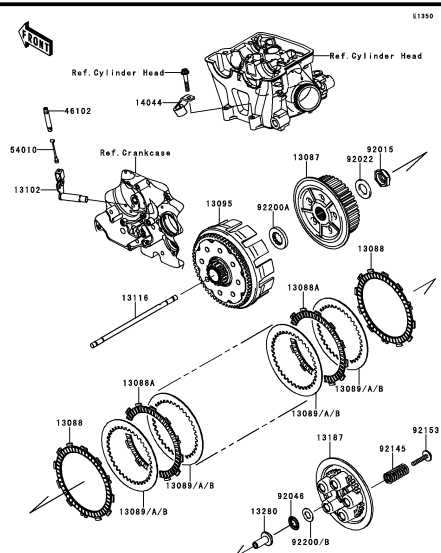
B-12 Clutch
