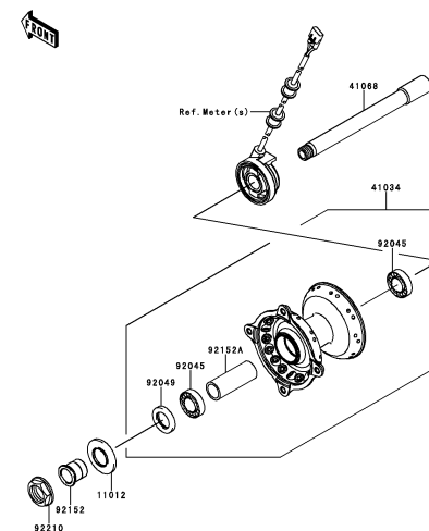
E-11 Front Hub
