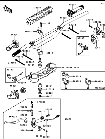
F-7 Handlebar
