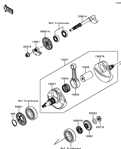
B-10 Crankshaft
