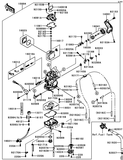
C-9 Carburetor(3/3)
