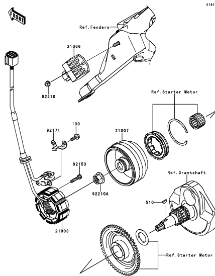
C-12 Generator
