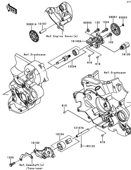
C-10 Oil Pump
