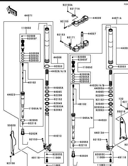
F-8 Front Fork(1/2)
