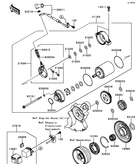
C-14 Starter Motor
