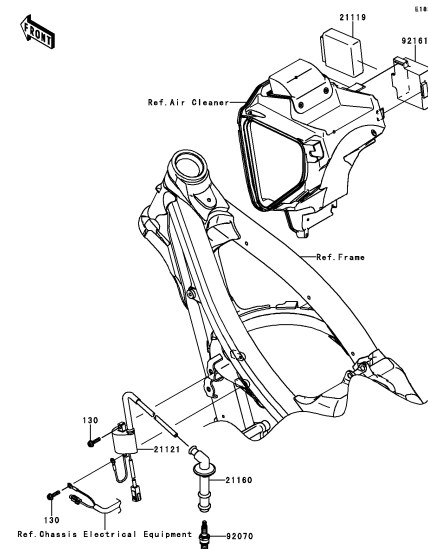
C-13 Ignition System
