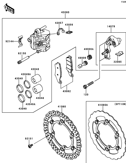
F-4 Front Brake
