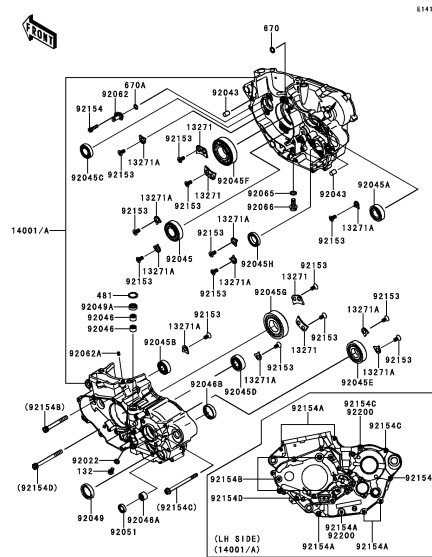
C-4 Crankcase
