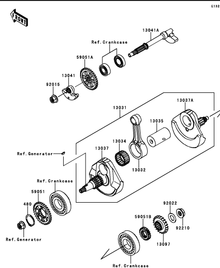
B-10 Crankshaft
