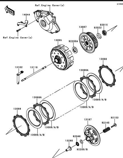
B-12 Clutch
