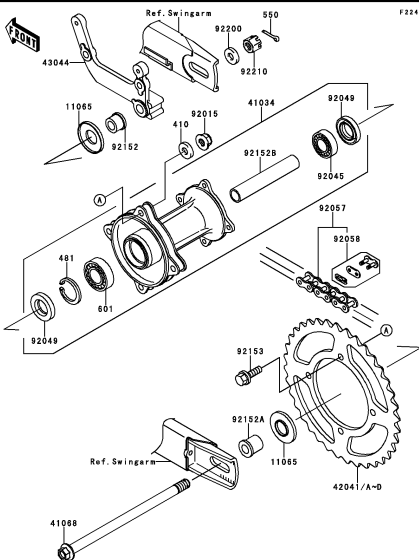
D-12 Rear Hub
