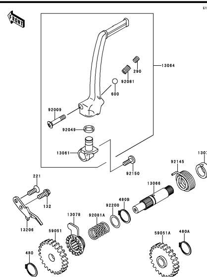
B-7 Kickstarter Mechanism
