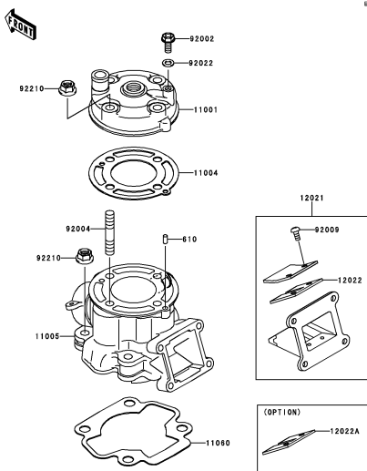
B-3 Cylinder Head/Cylinder
