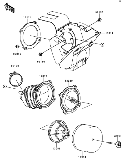
B-4 Air Cleaner
