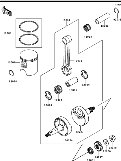
B-6 Crankshaft/Piston(s)
