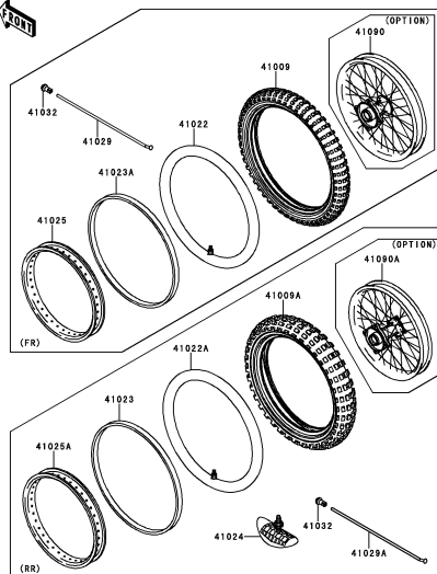
D-10 Tires
