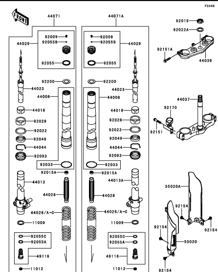
E-8 Front Fork(1/2)
