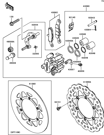
E-4 Front Brake
