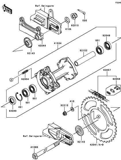
D-12 Rear Hub
