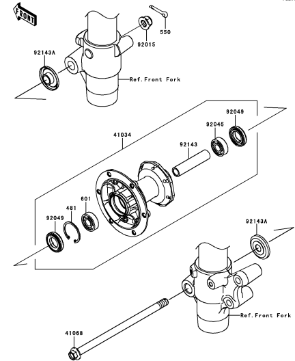
D-11 Front Hub
