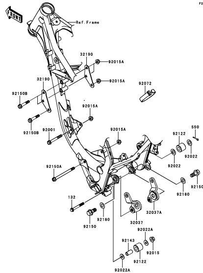
D-4 Engine Mount
