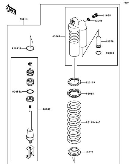
D-14 Shock Absorber(s)
