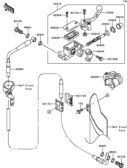
E-3 Front Master Cylinder
