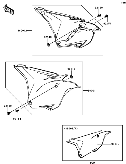
E-13 Side Covers
