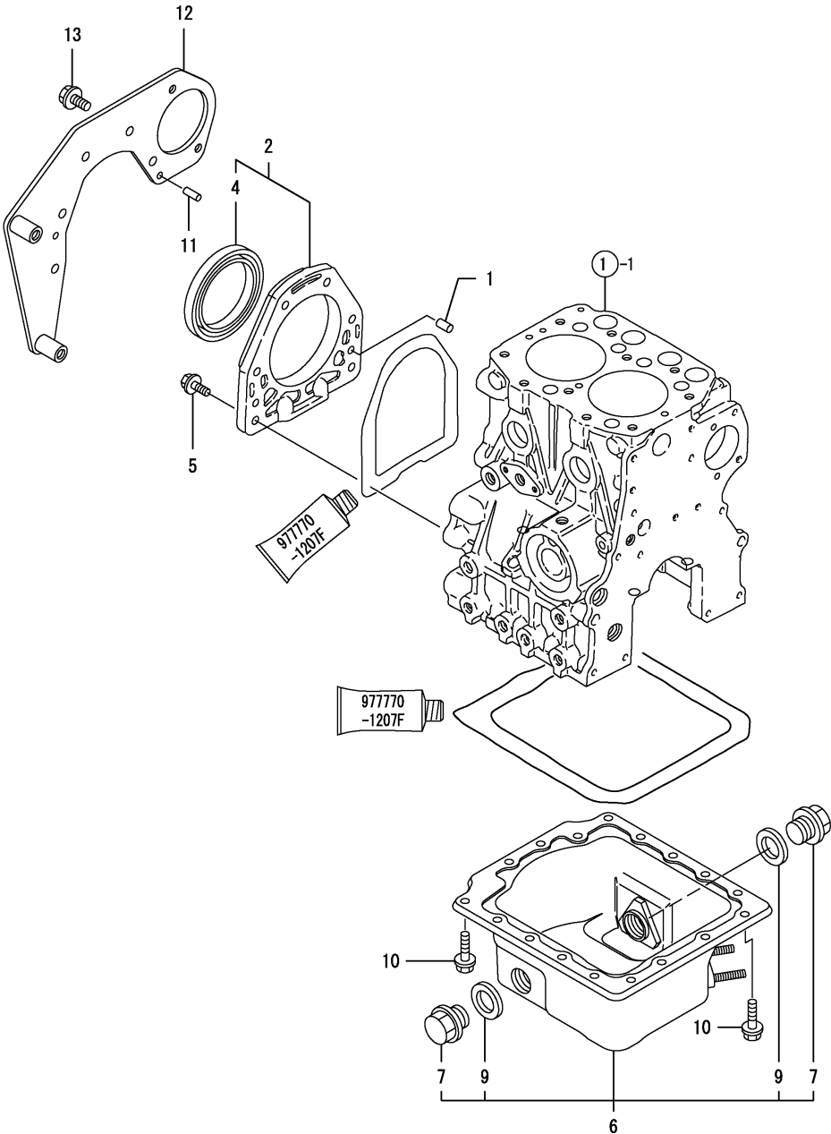
Fig.3. OIL SUMP
