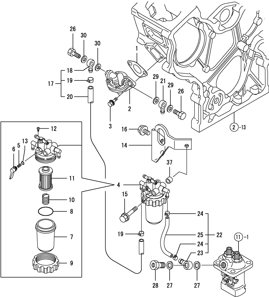
Fig.14. FUEL LINE
