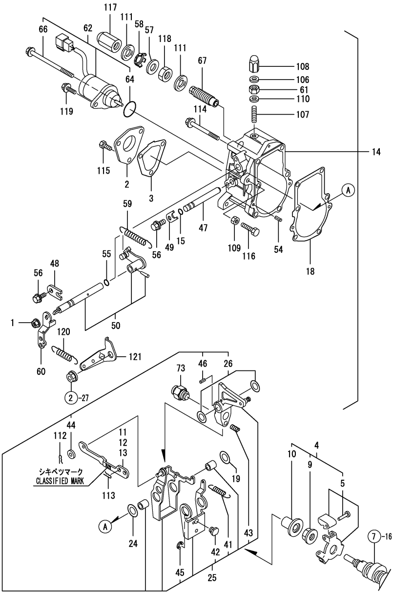
Fig.12. GOVERNOR
