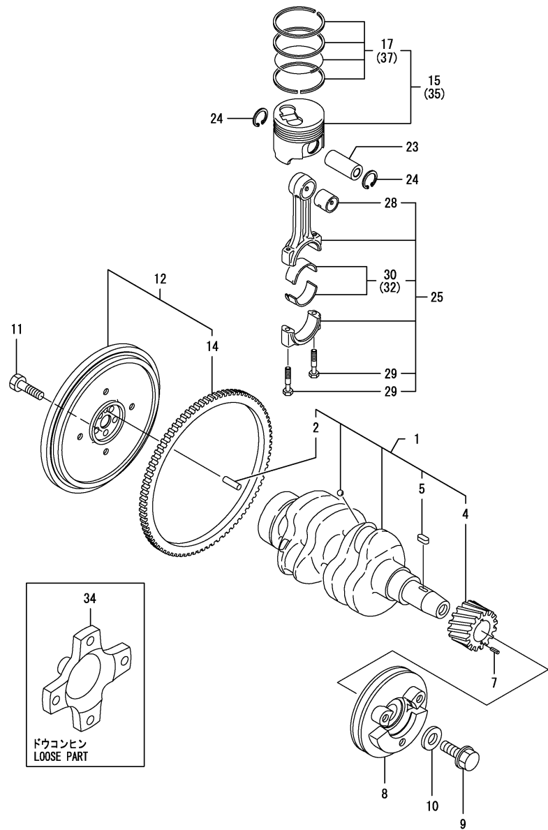
Fig.8. CRANKSHAFT & PISTON
