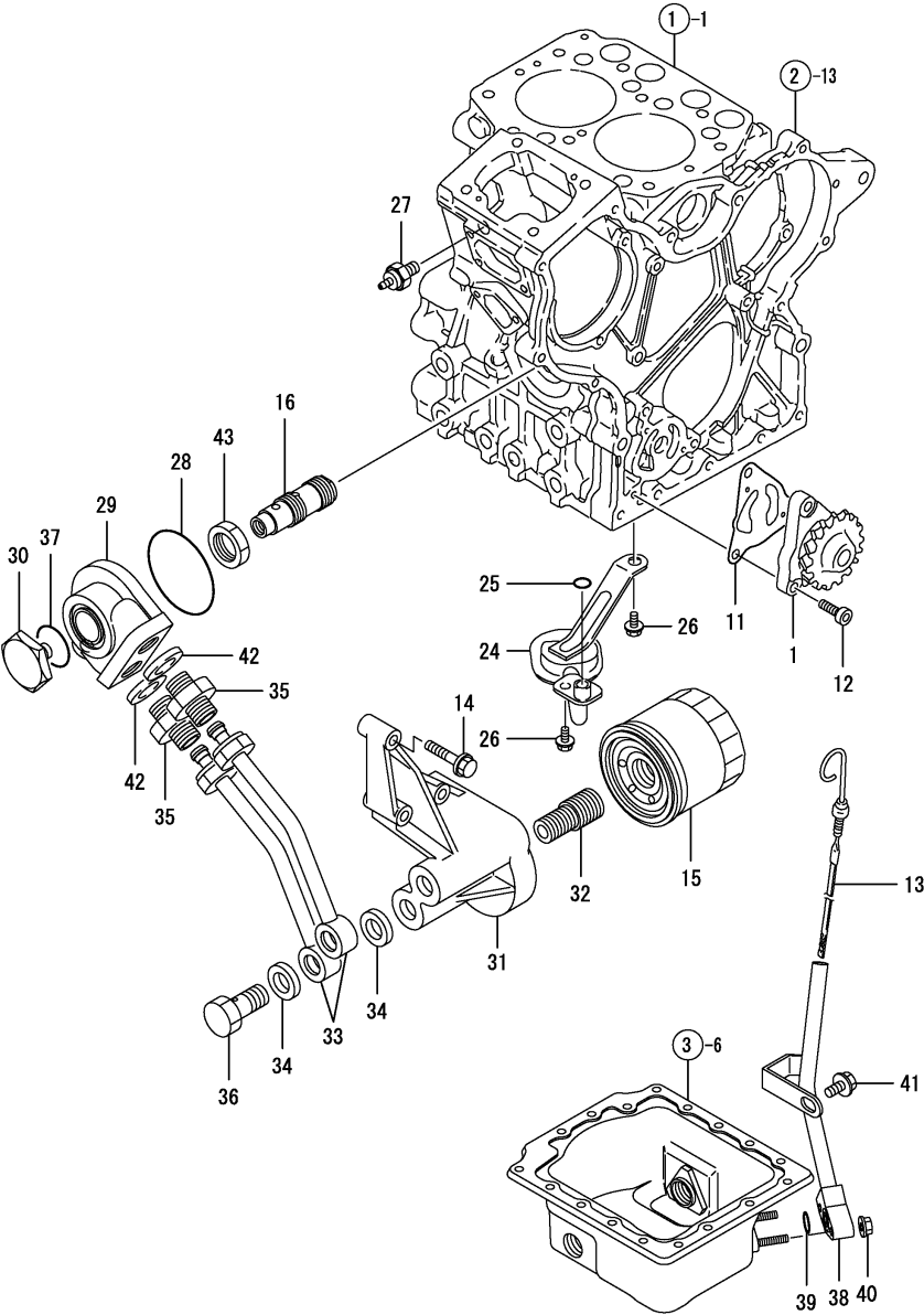
Fig.9. LUB.OIL SYSTEM
