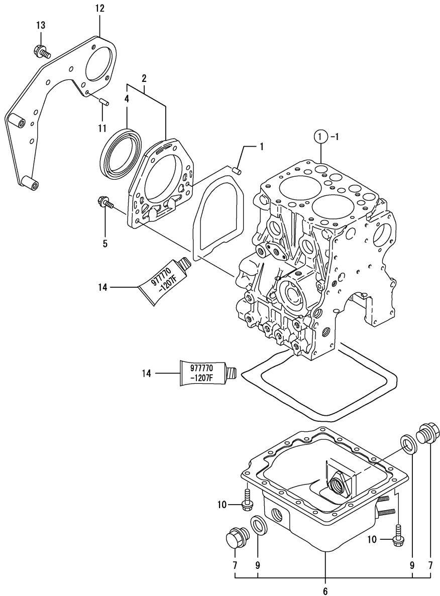
Fig.3. OIL SUMP
