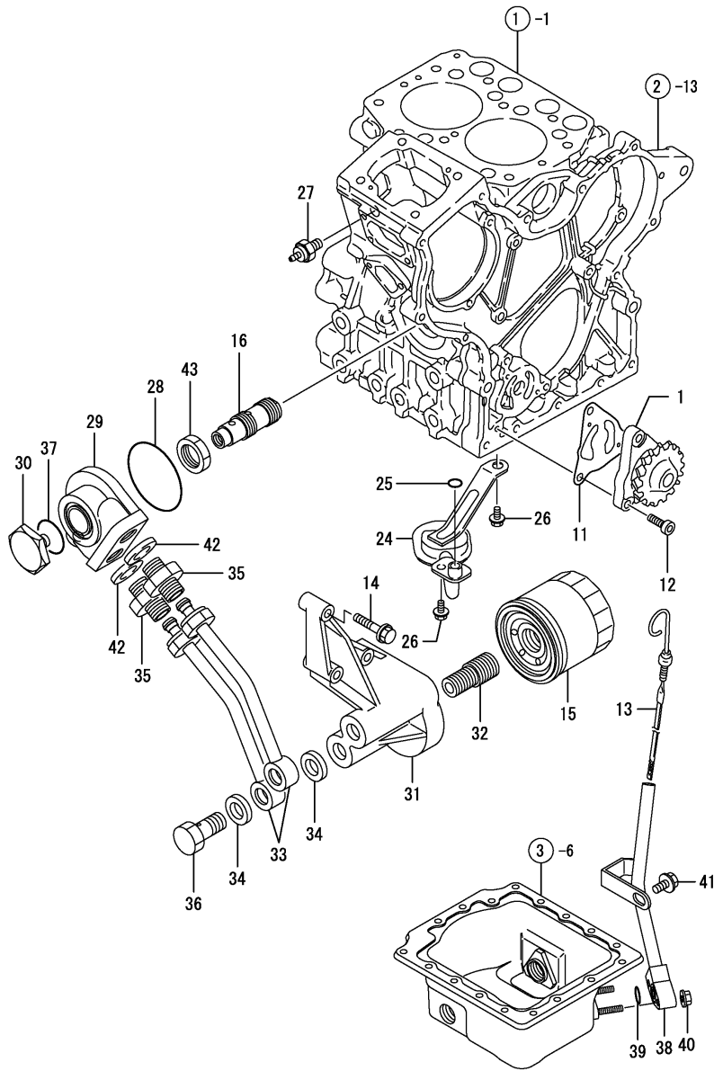
Fig.9. LUB.OIL SYSTEM
