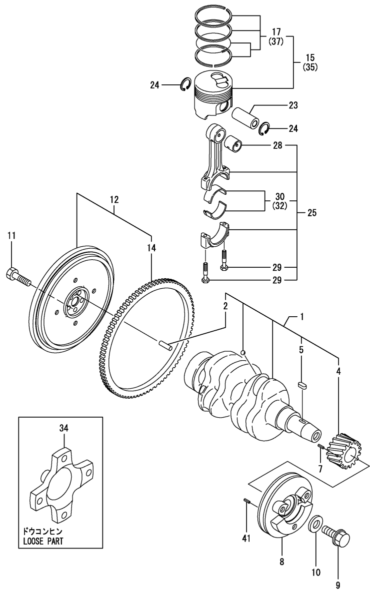
Fig.8. CRANKSHAFT & PISTON
