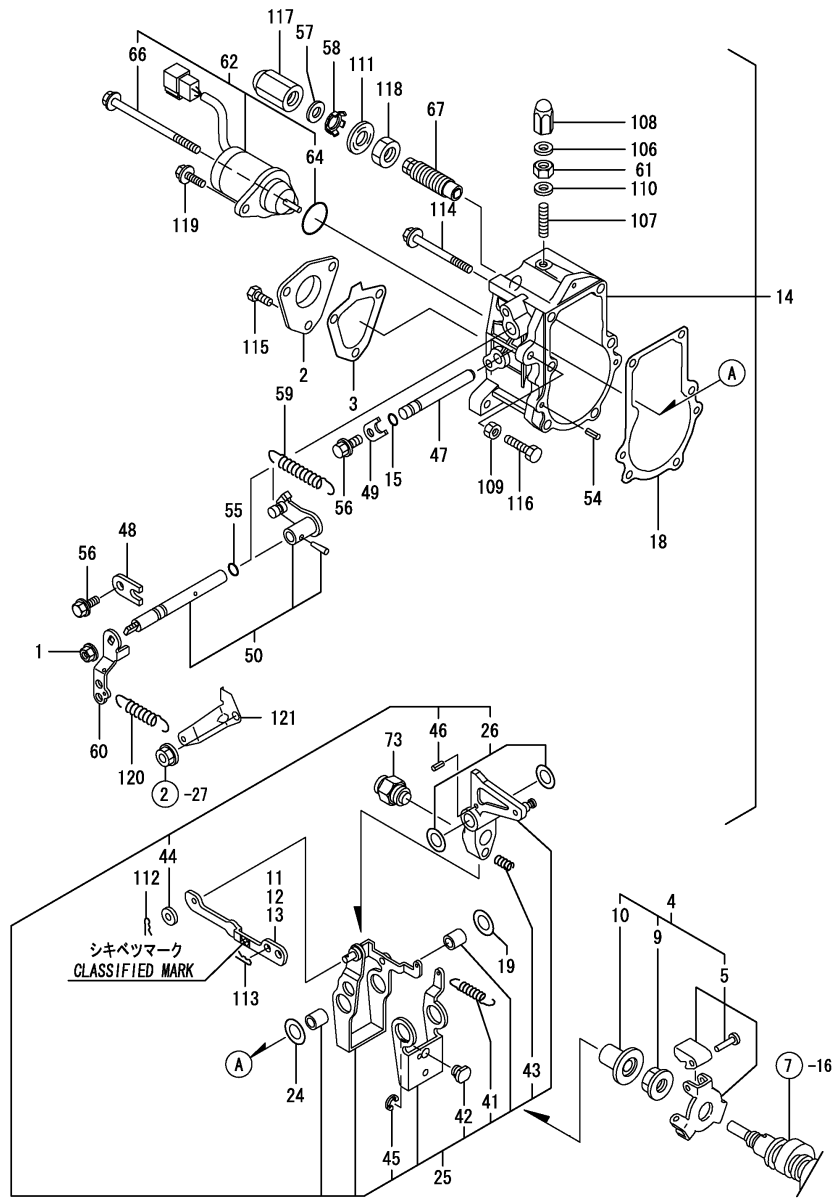
Fig.12. GOVERNOR
