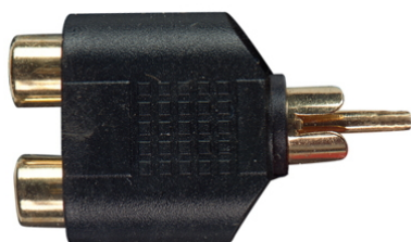
AC-2CFCMH 44 kr One-piece audio adaptor - Dual Fem. phono socket / 1 male phono socket - ROHS Compliant - 2 pcs in blister packaging
